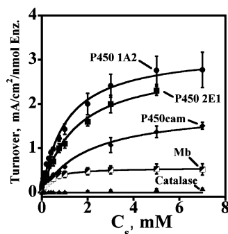
Figure 8. Michaelis–Menten fits (eq 4) of relative turnover rate ( I_L/T ) vs t-BuOOH concentration for cyt P450, myoglobin, and catalase films. Points are experimental data, and solid lines represent the best fit of eq 4 by nonlinear regression. RDV parameters are as in Figure 7.
