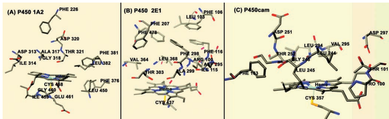
Figure 9. Heme structures with distal and proximal region amino acid residues for (A) cyt P450 1A2 (PDB:2HI4), 51 (B) cyt P450 2E1 (PDB:3E4E), 52 and (C) cyt P450cam (PDB:2CPP). 53
