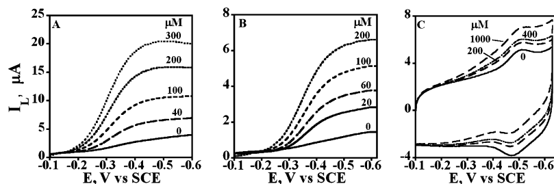
Figure 7. Representative steady state RDVs at 1000 rpm for protein films on PG electrodes for t-BuOOH reduction in anaerobic 50 mM potassium phosphate buffer + 0.1 M NaCl, pH 7.0 at 25 °C. RDVs for increasing t-BuOOH concentration (in \mu\text{M} ) for (A) PEI/(PSS/P450 2E1) 4 , (B) PSS/(PEI/P450cam) 4 , and (C) PSS/(PEI/catalase) 4 films.
